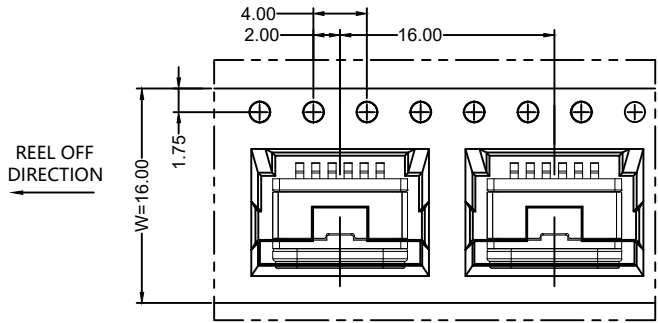
DETAIL X
