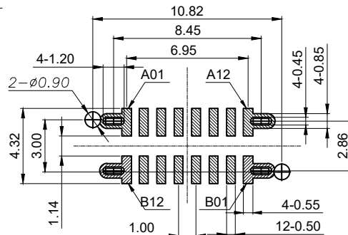
RECOMMENDED P.C.B. LAYOUT (俯视图)
